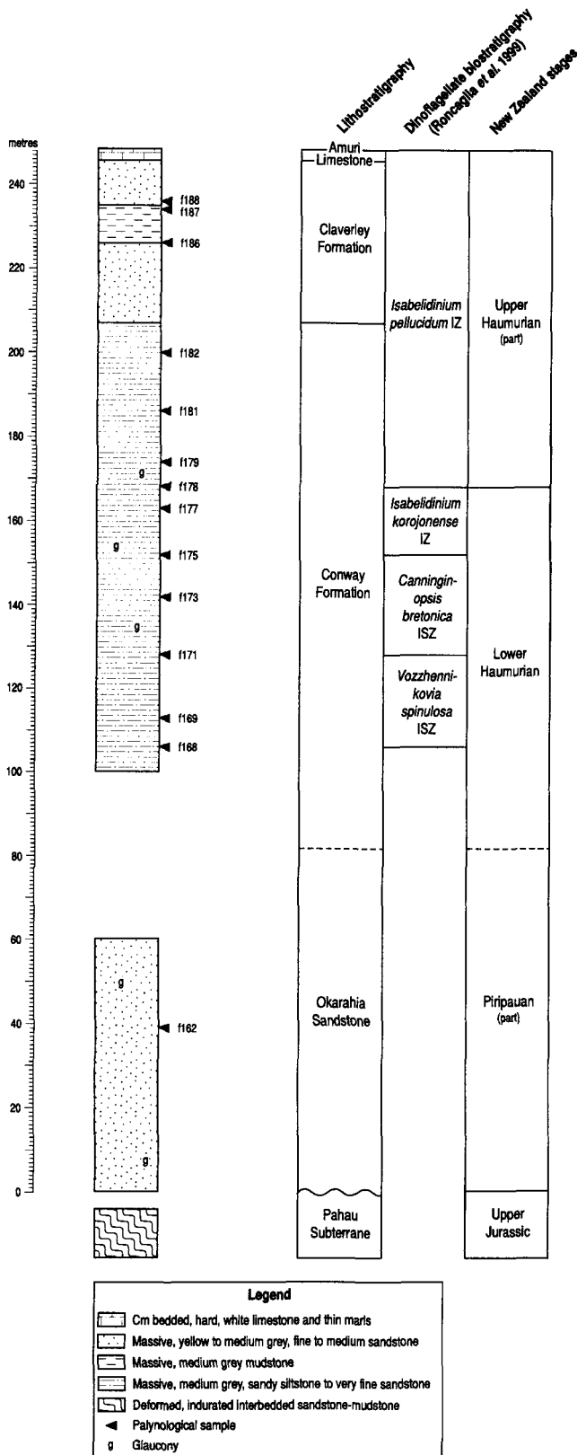
Fig. 7 Log of the Conway River railway cutting section, showing sample horizons and summarising biostratigraphic results. All fossil localities are registered in the Fossil Record File for map sheet O32, housed in the Department of Earth Sciences, University of Canterbury, Christchurch.
