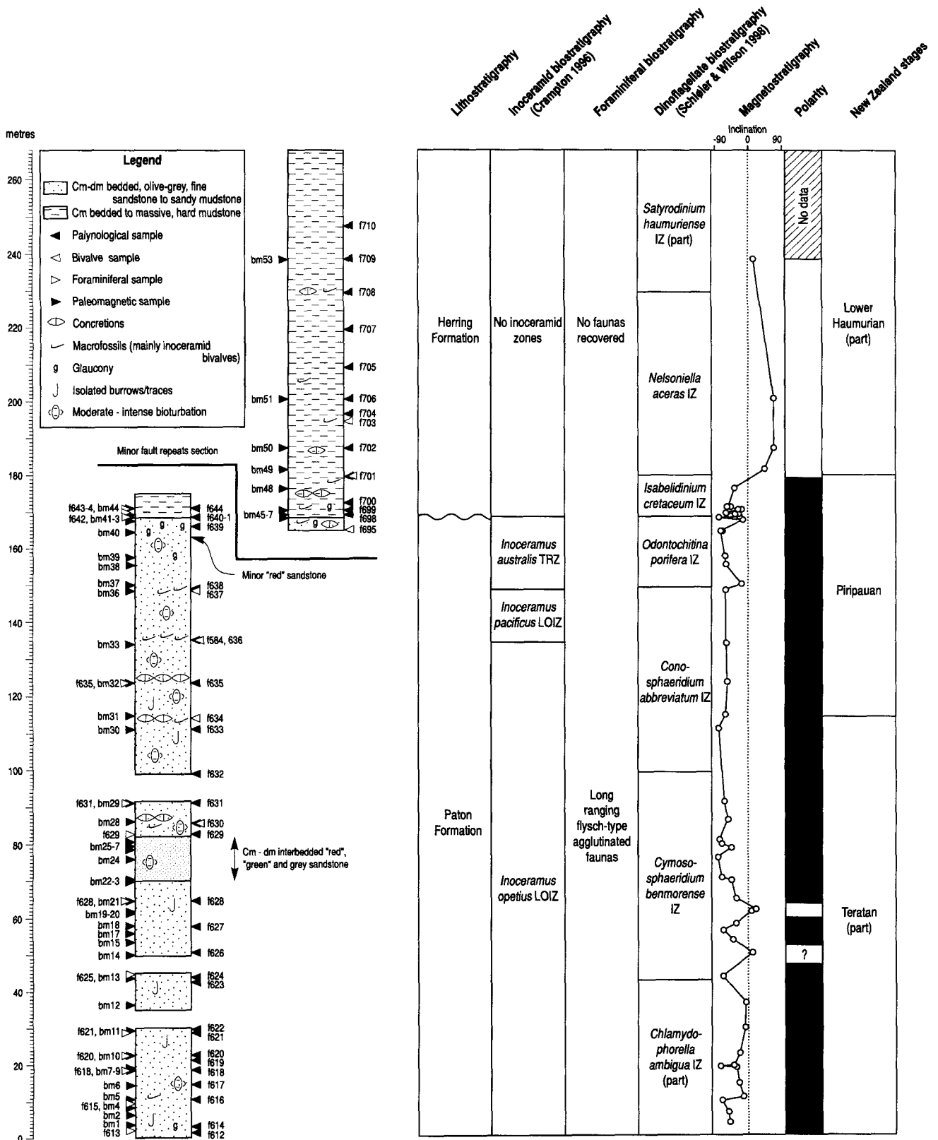
Fig. 5 Log of the Ben More Stream tributary section, showing sample horizons and summarising biostratigraphic and magnetostratigraphic results. All fossil localities are registered in the Fossil Record File for map sheet P30, housed in the Department of Earth Sciences, University of Canterbury, Christchurch.
