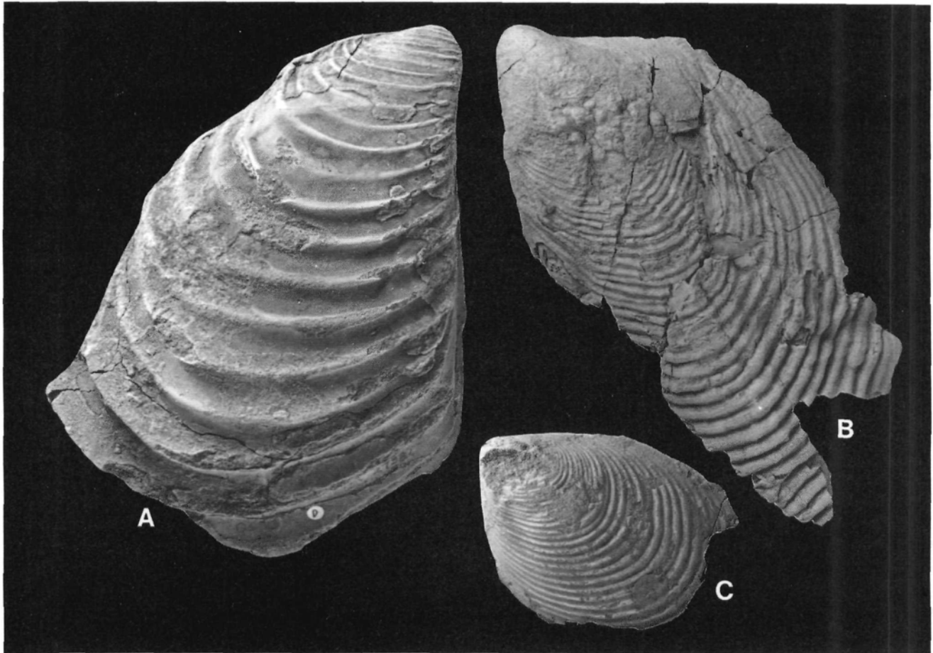
Fig. 8 Piriapuan (uppermost Coniacian to middle Santonian) inoceramid bivalves from the northeastern part of the South Island, New Zealand. All specimens \times 0.66 and whitened with ammonium chloride. Specimens prefixed "IGNS" are housed at the IGNS, Lower Hutt. The specimen prefixed "BMNH" is housed at the Natural History Museum, London. A , Inoceramus australis Woods (lectotype). IGNS TM2738, GS13, O32/f8025, Haumuri Bluff. Right valve, internal mould with patches of shell preserved. B , Inoceramus pacificus nanakius Crampton (holotype). IGNS TM7974, GS15053, P30/f584, Ben More Stream section. Left valve, prismatic shell preserved. C , Inoceramus pacificus pacificus Woods. BMNH LL9789, O32/f- (not registered), Haumuri Bluff. Left valve, internal mould.
